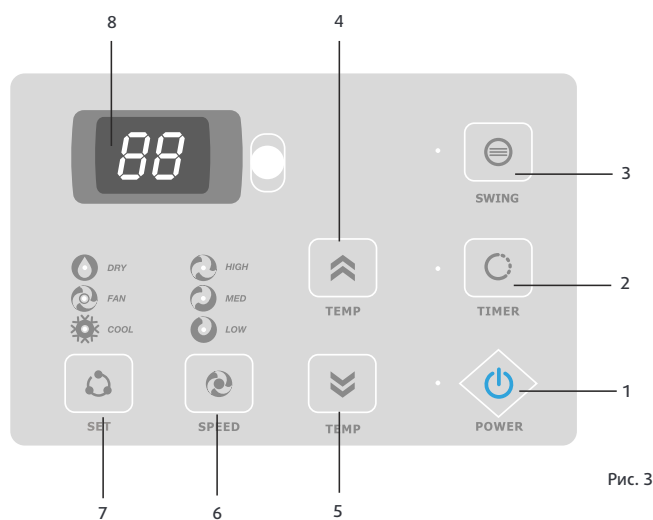
Control panel of AC TIM 09HW1E, AC TIM 12HW1E.
