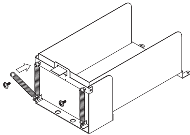
Figure 12 – The process of spring replacement
