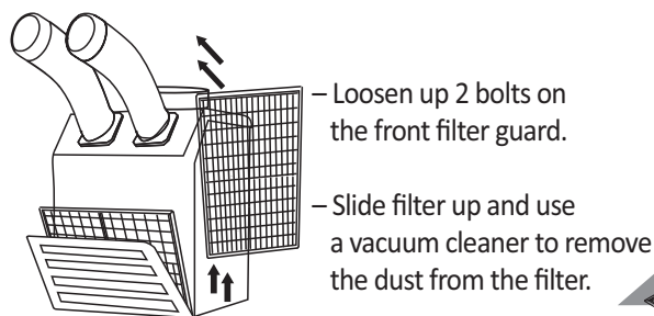
Figure 10 – Removing Filters
