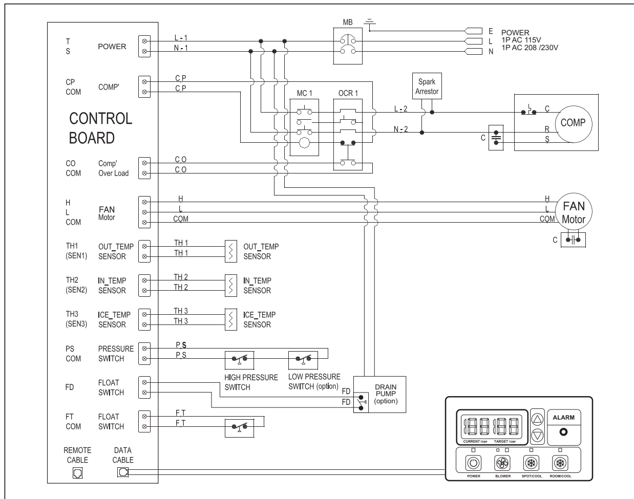
Figure 13 - Circuit Wiring Diagram (WPC-3000,5000)
