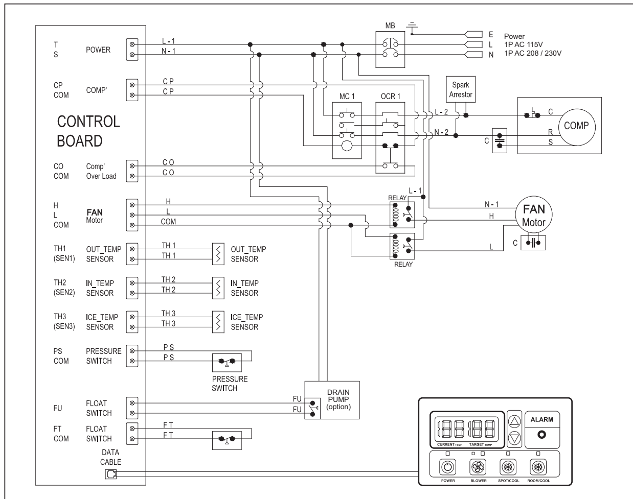
Figure 14 - Circuit Wiring Diagram (WPC-4000)
