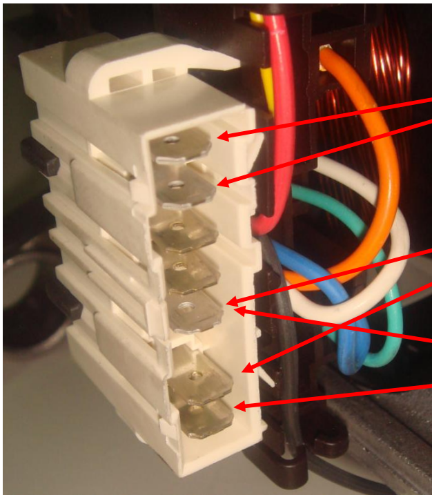
Motor Socket Terminals
